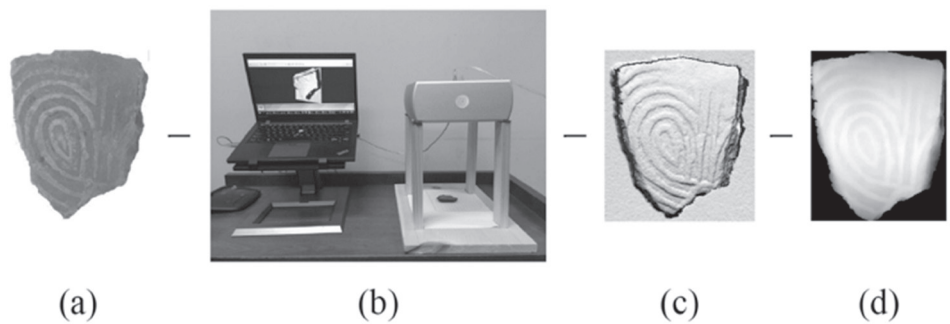
Figure 5: An illustration of scanning sherds for depth images. (a) RGB image of a sherd. (b) Setup of a 3D scanner. (c) 3D point cloud of the sherd surface obtained by the 3D scanner. (d) Depth image of the sherd surface: pixel intensity represents the depth value at a location.
